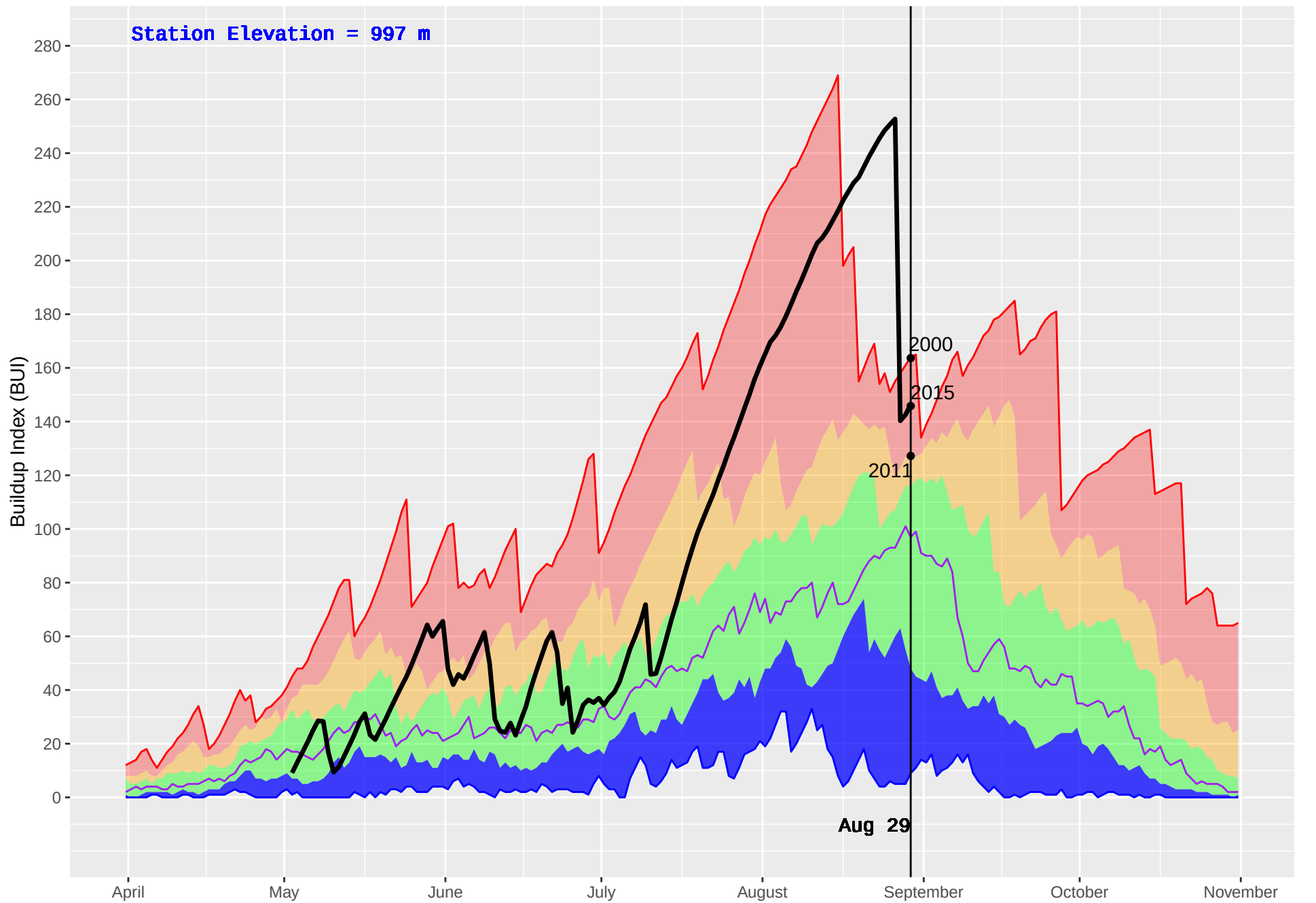
SMALLWOOD (404) : Historical (1991–2016) and Current (2018) Daily Buildup Index (BUI)
