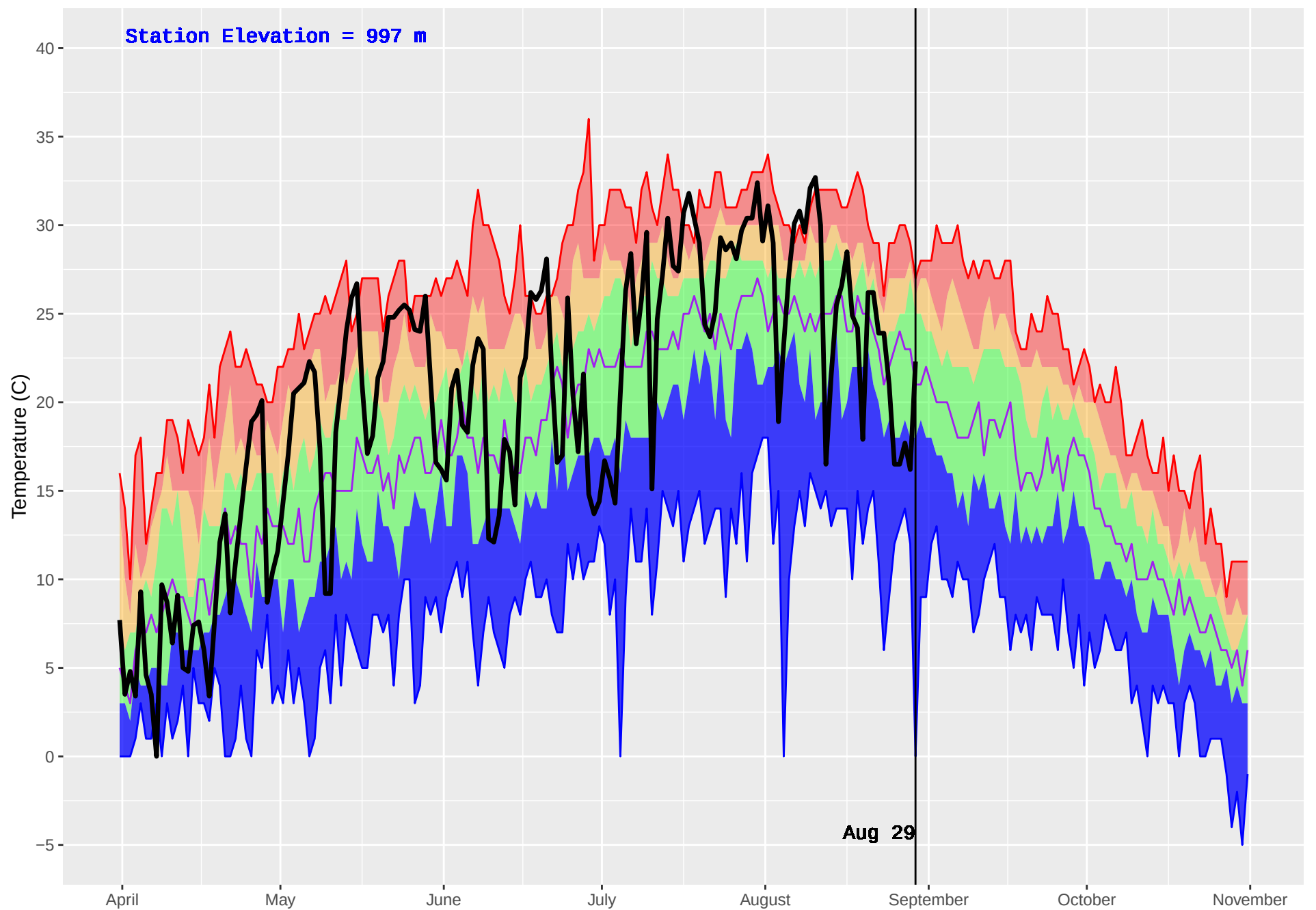
SMALLWOOD (404) : Historical (1991–2016) and Current (2018) Daily Temperature
