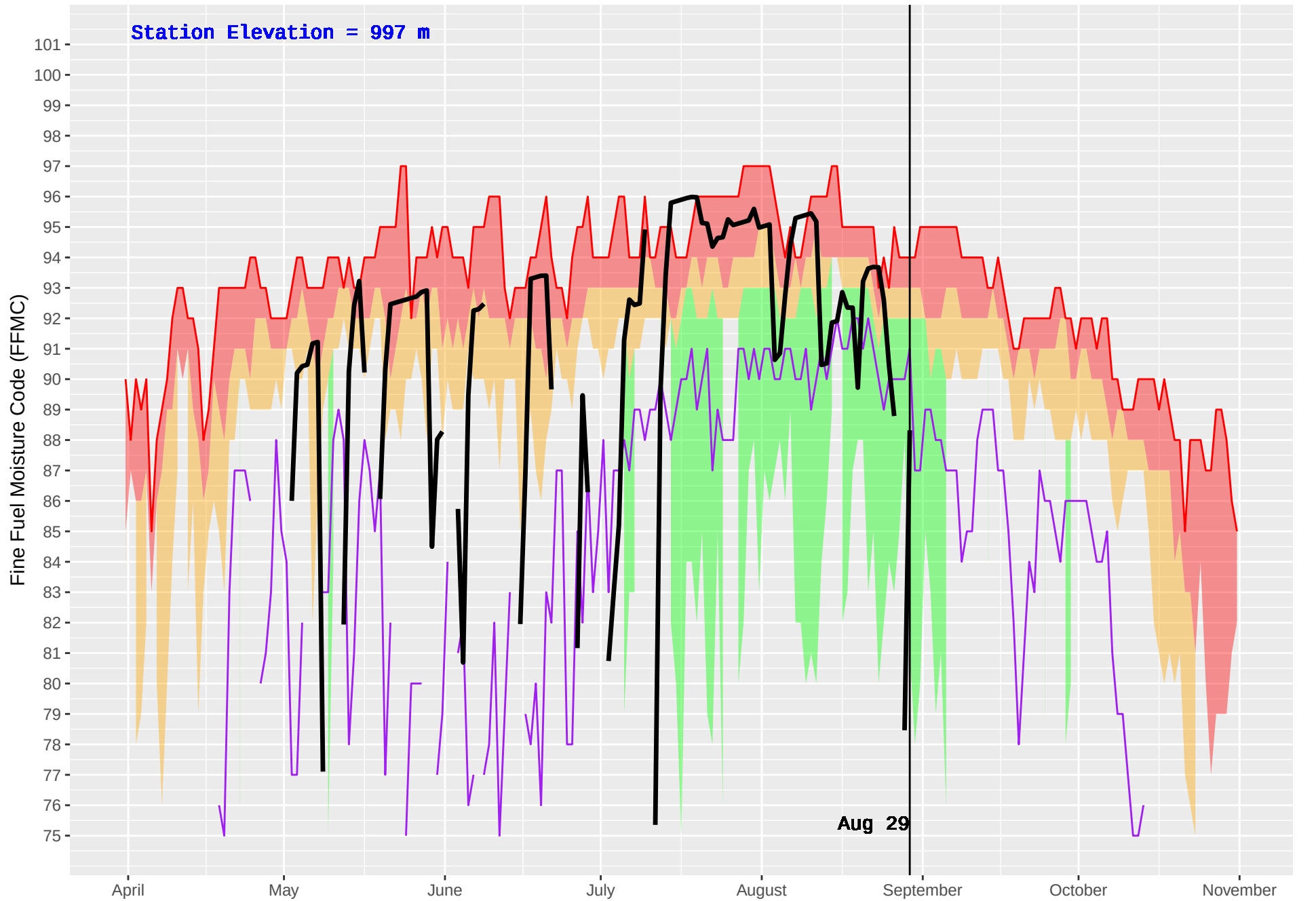
SMALLWOOD (404) : Historical (1991–2016) and Current (2018) Daily Fine Fuel Moisture Code (FFMC)
