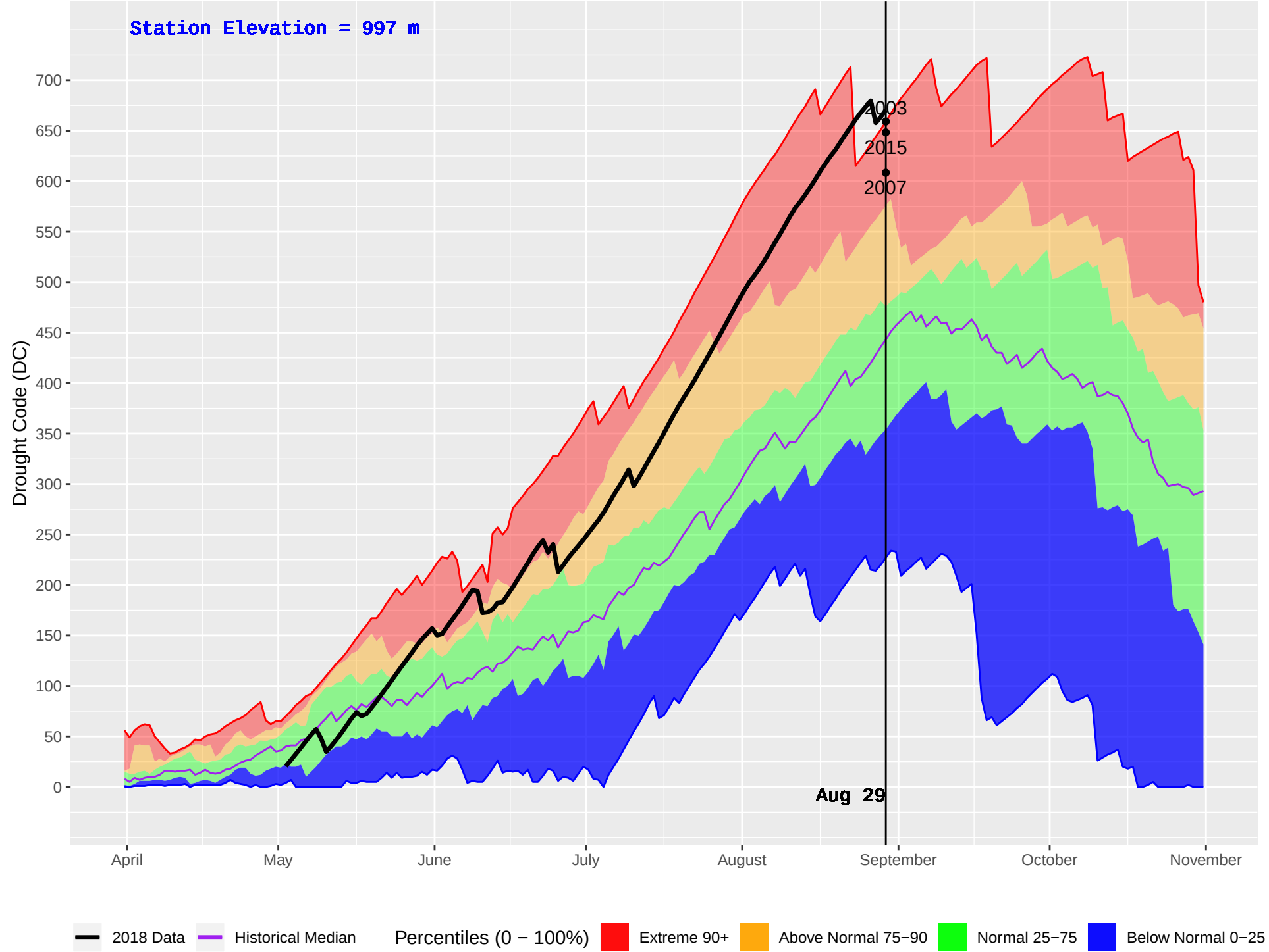
SMALLWOOD (404) : Historical (1991–2016) and Current (2018) Daily Drought Code (DC)
