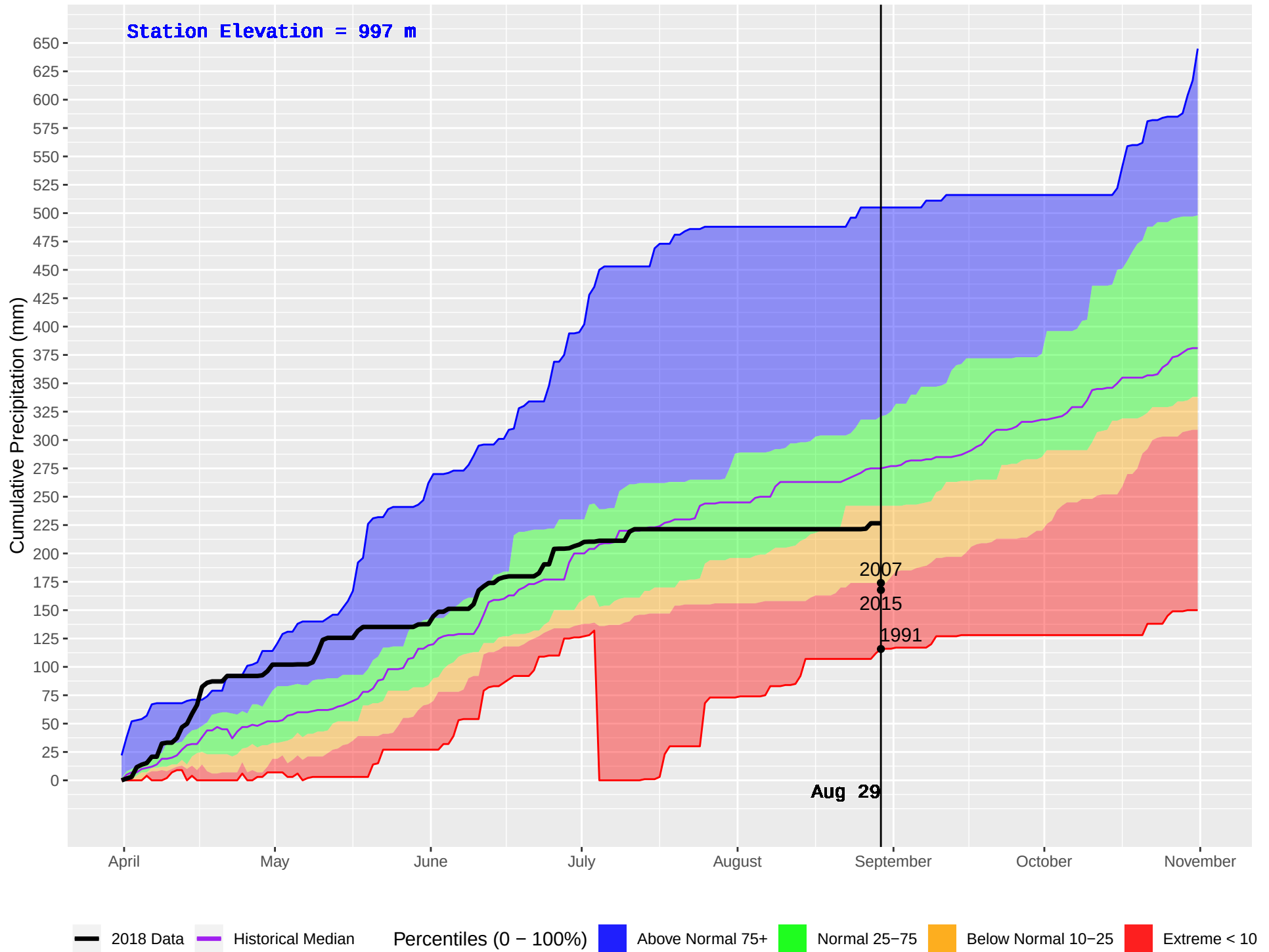
SMALLWOOD (404) : Historical (1991–2016) and Current (2018) Daily Cumulative Precipitation
