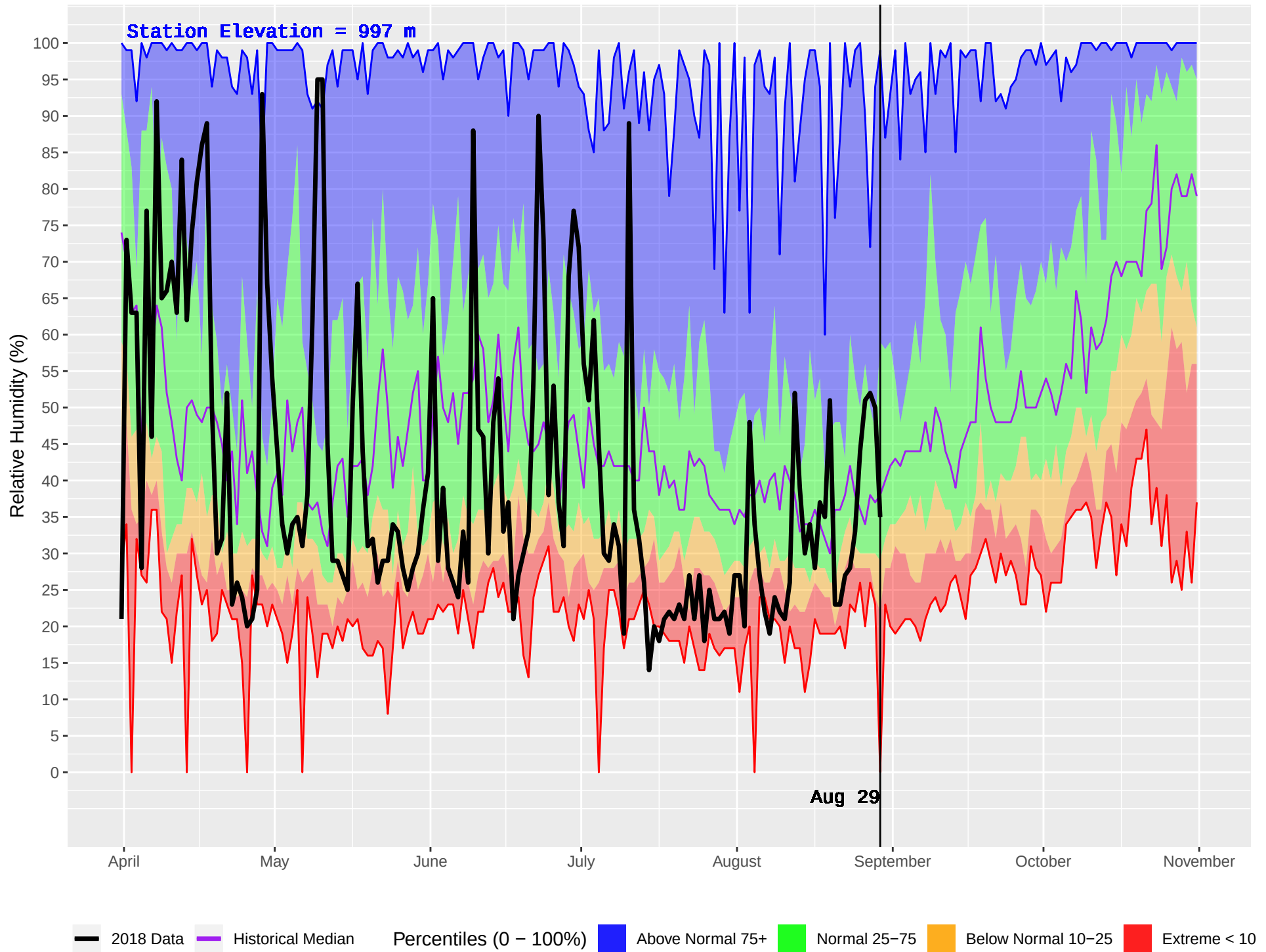
SMALLWOOD (404) : Historical (1991–2016) and Current (2018) Daily Relative Humidity
