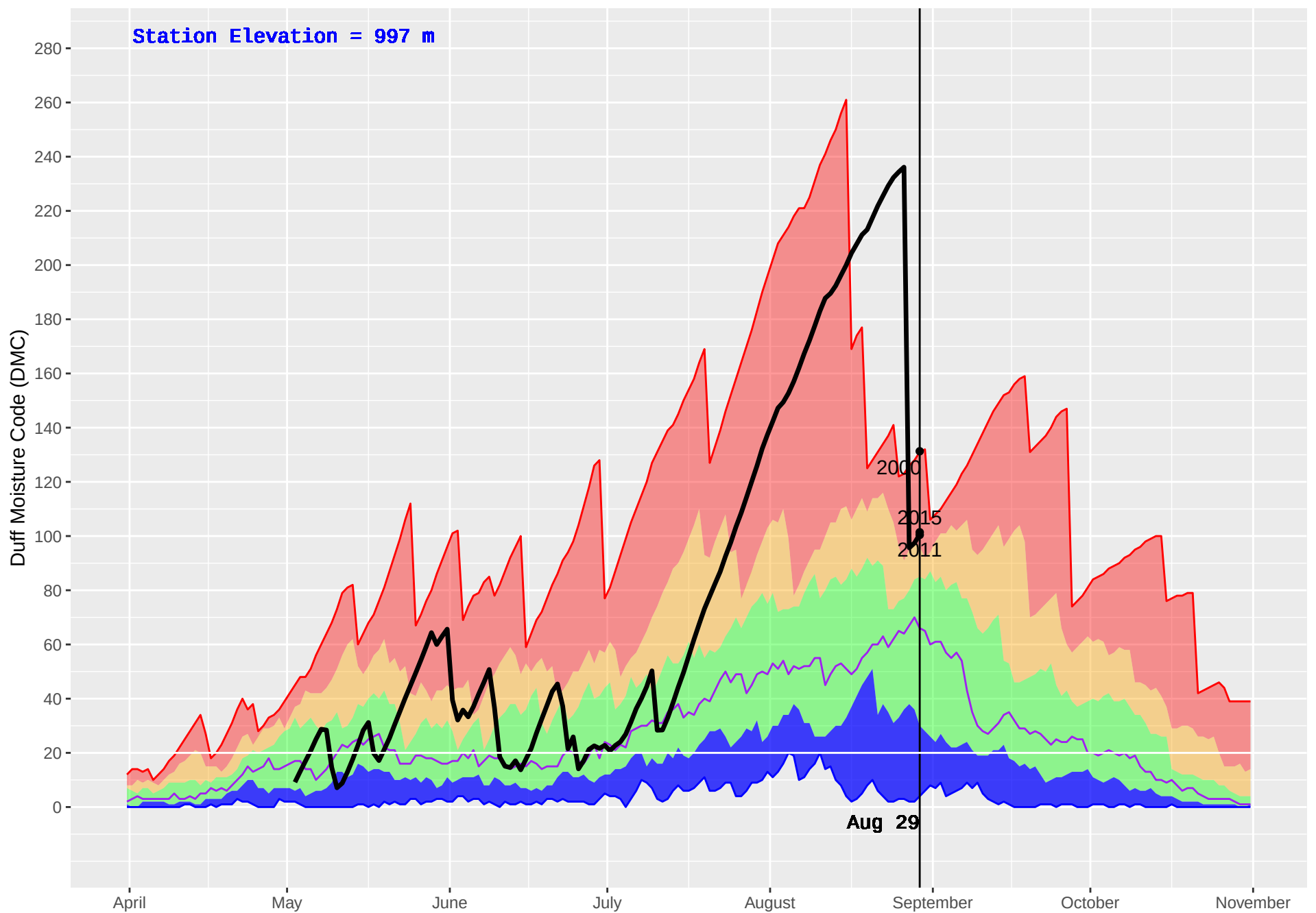
SMALLWOOD (404) : Historical (1991–2016) and Current (2018) Daily Duff Moisture Code (DMC)
